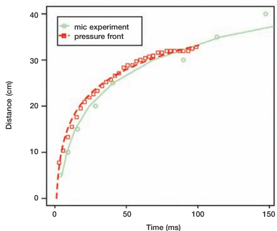
Figure 7. Microphone experiments correlate well with pressure front simulations.
