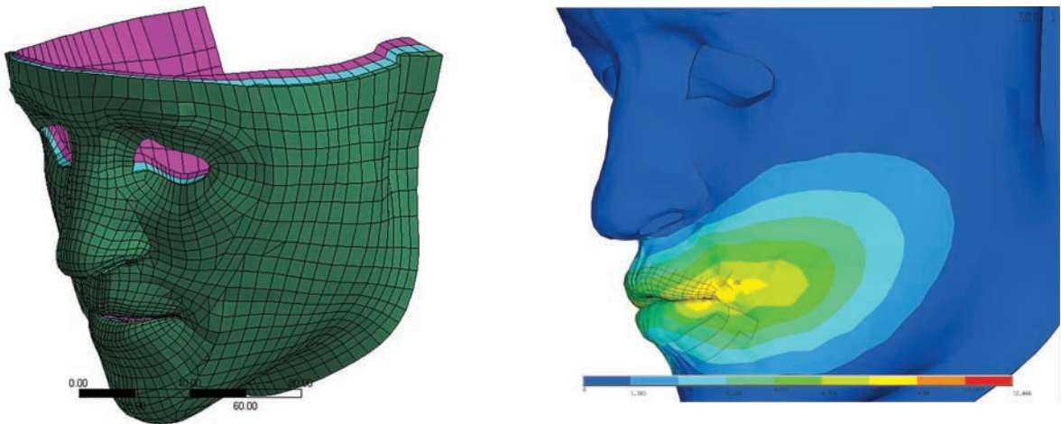
Figure 2. Manually designed 3-D finite element mesh consists of three layers of full and degenerated ANSYS SOLID185 hexahedral elements (left); round-shaped lips with a protrusion make the sound “ou” (right).
