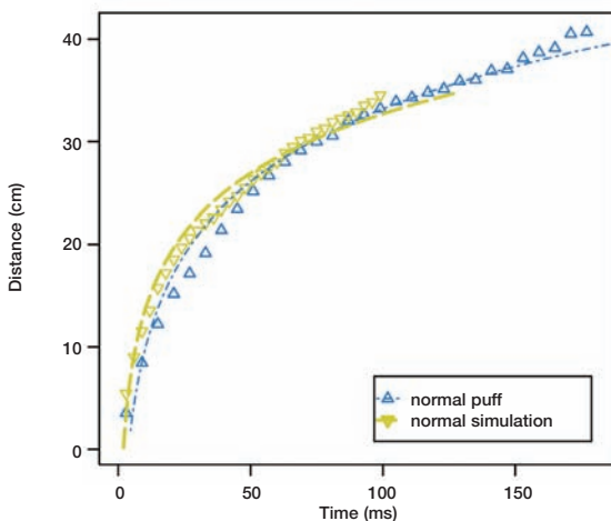
Figure 6. Comparison between high-speed video and particle front simulation
